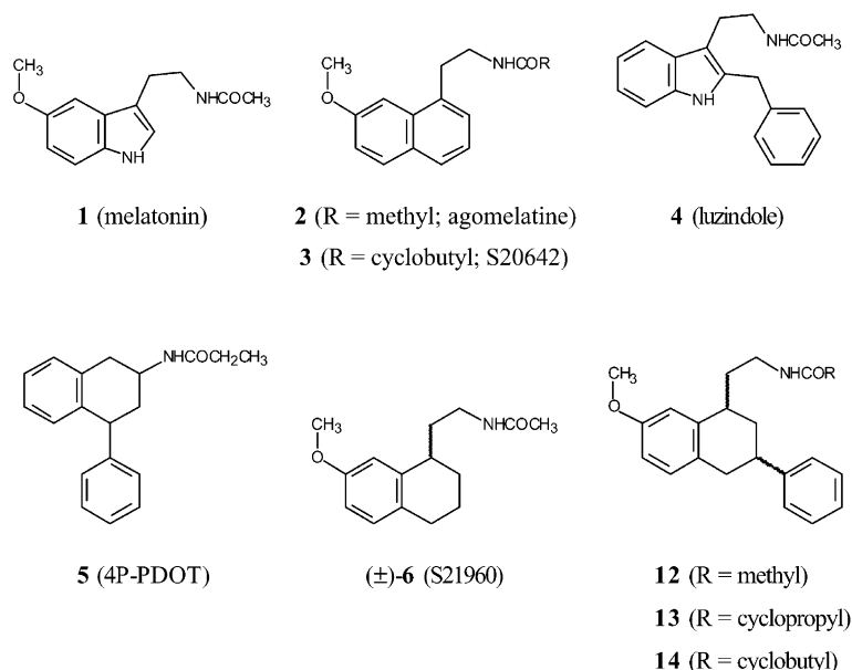
Chart 1. Chemical structures of melatonin ligands.
