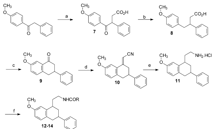
Scheme 1. Synthesis of compounds 12–14 . Reagents: (a) (i) \text{BrCH}_2\text{COOCH}_3 , NaH, DMF; (ii) NaOH, methanol, water; (b) (\text{C}_2\text{H}_5)_3\text{SiH} , \text{CF}_3\text{COOH} ; (c) Polyphosphoric acid; (d) (\text{C}_2\text{H}_5\text{O})_2\text{P}(\text{O})\text{CH}_2\text{CN} , NaH, anhydrous THF; (e) \text{H}_2 , Raney nickel, ethanol, \text{NH}_2\cdot\text{HCl} (g); (f) \text{RCOCl} , \text{K}_2\text{CO}_3 , chloroform, water.
